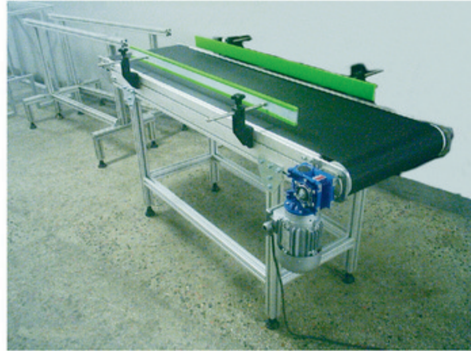
PVC Flat Belt Conveyor
